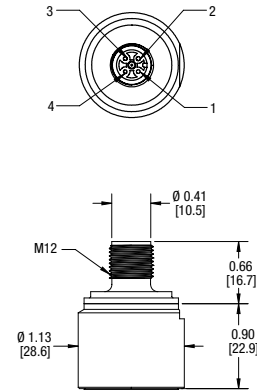
M12 CODE: 00EW
